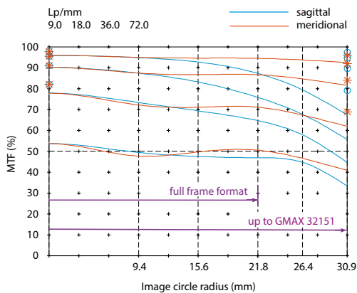
MTF of d.fine HR-M 2.8/80 @ ratio 0.2 and f-stop = 2.8
